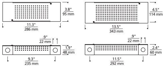
60W 0-10V ENCLOSURE
